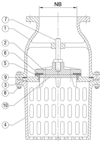
LIFT TYPE FOOT VALVE
