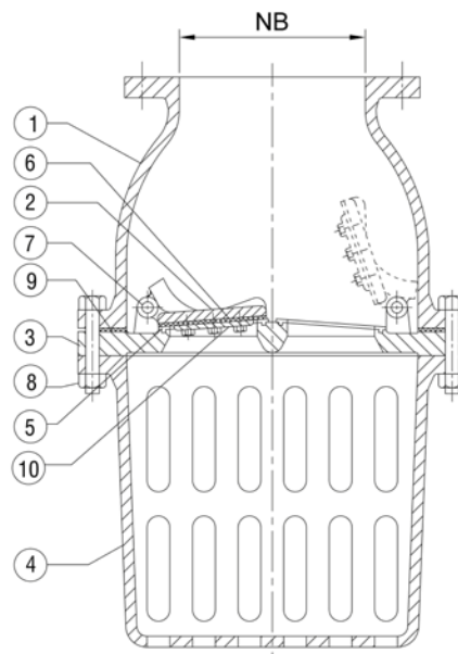
SWING TYPE FOOT VALVE
